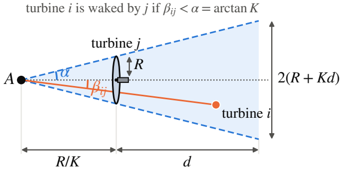
Fig. 3: Wake half cone of turbine j (schematic, K exaggerated). The virtual vertex A lies a distance R/K upstream of the rotor, the half-cone angle is \alpha = \arctan(K) , and a downstream turbine i lies in the wake of j when \beta_{ij} < \alpha .
