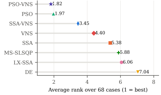
Fig. 1. Average rank of the eight methods over the 68 benchmark cases (1 = best; ranking rule of Table I).
