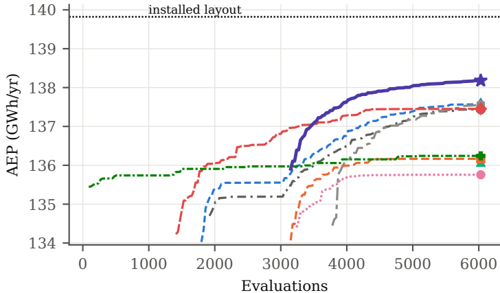
Horns Rev 1, 16 turbines: median best feasible AEP
