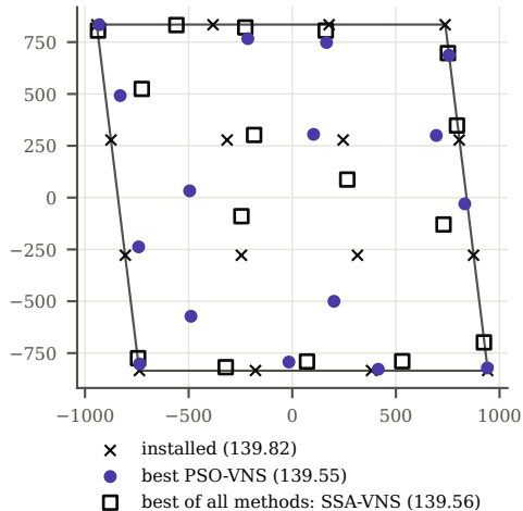
Layouts (m); AEP in GWh/yr
