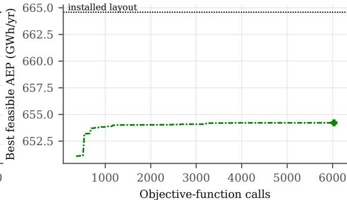
Horns Rev 1, 80 turbines
