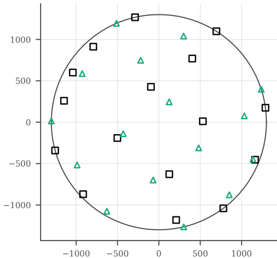
IEA37 CS1, 16 turbines (m)
