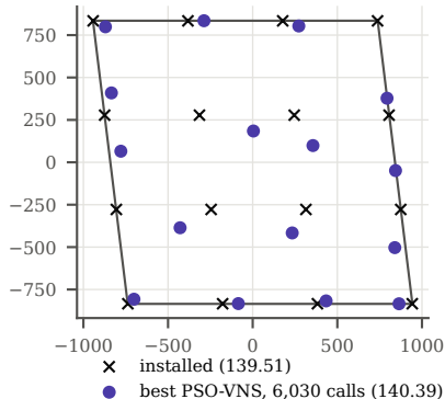
Horns Rev 1, 16 turbines (AEP in GWh/yr)
