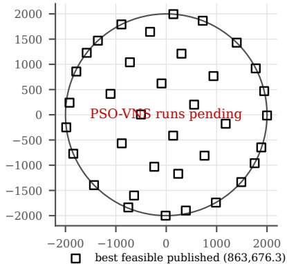
IEA37 CS1, 36 turbines (AEP in MWh)
