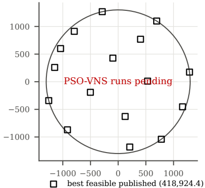
IEA37 CS1, 16 turbines (AEP in MWh)
