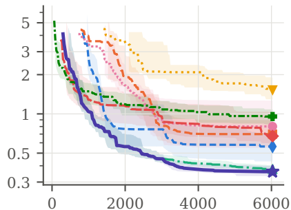
Data Set II, r = 750 m, N = 8
