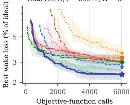
Data Set II, r = 500 m, N = 6
