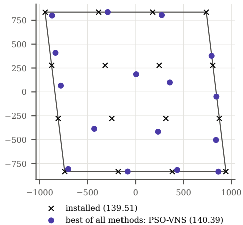
Layouts (m); AEP in GWh/yr
