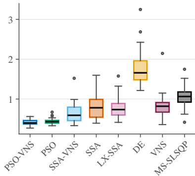
Data Set I, r = 1000 m, N = 10
