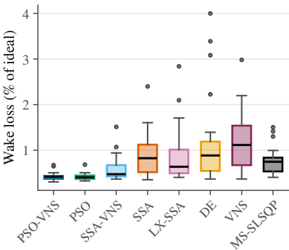
Data Set I, r = 500 m, N = 6
