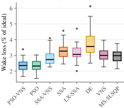
Data Set II, r = 500 m, N = 6
