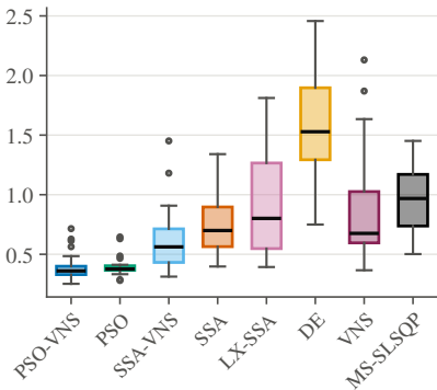
Data Set I, r = 750 m, N = 8
