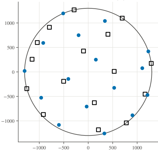
IEA37 CS1, 16 turbines (m)
