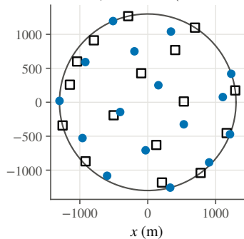
IEA37 CS1, 16 turbines (AEP in MWh)
