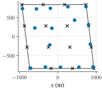
Horns Rev 1, 16 turbines (AEP in GWh/yr)
