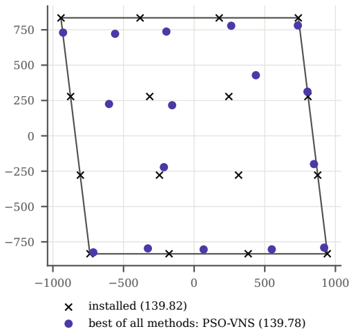
Layouts (m); AEP in GWh/yr
