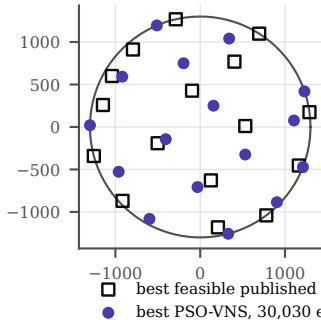
IEA37 CS1, 16 turbines (AEP in MWh)
