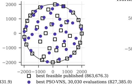
IEA37 CS1, 36 turbines (AEP in MWh)
