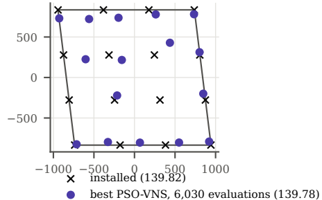
Horns Rev 1, 16 turbines (AEP in GWh/yr)
