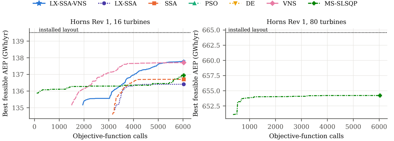
Fig. 12: Horns Rev 1 site case: median best feasible AEP versus objective calls (16-turbine block: 30 runs; 80-turbine farm: 10 runs); dotted line: installed layout. Only MS-SLSQP finds feasible layouts for the 80-turbine farm.
