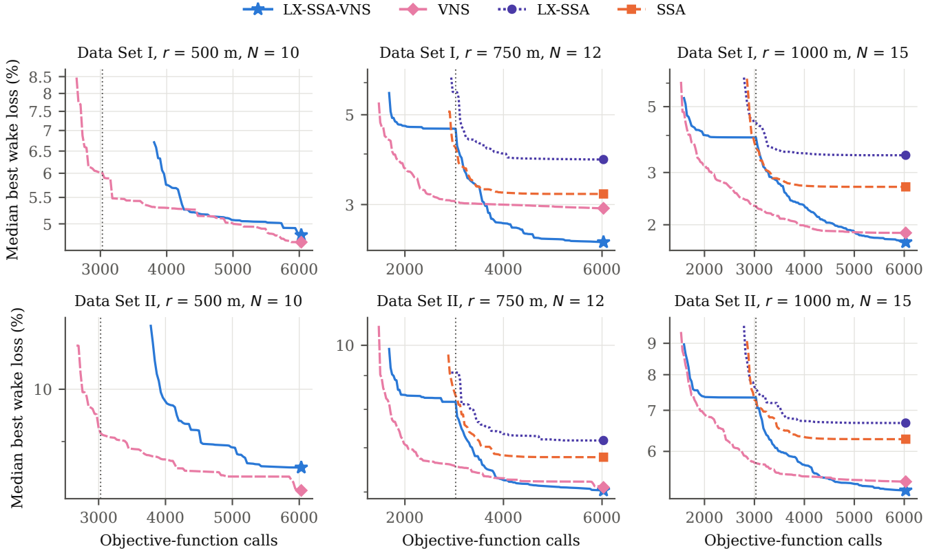
Fig. 10: Component ablation, largest turbine count of each farm: median best feasible wake loss over 30 runs versus objective calls for SSA, LX-SSA, VNS and LX-SSA-VNS (dotted vertical line: switch from LX-SSA to VNS in the hybrid at 3,030 calls).
