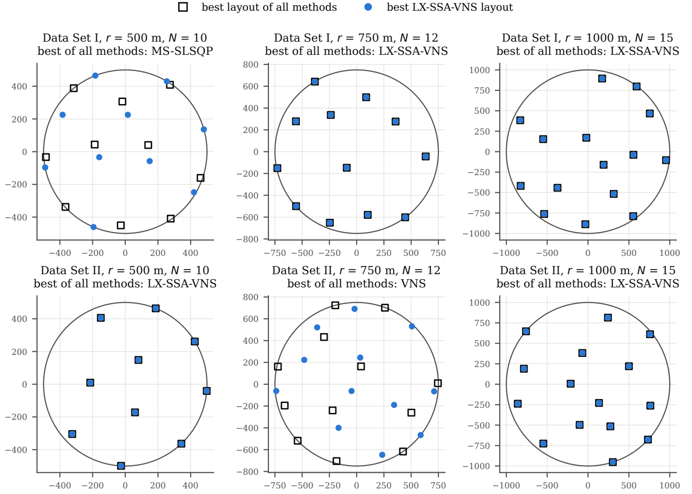
Fig. 11: Best layouts for the largest turbine count of each farm: best LX-SSA-VNS run (filled blue circles) and best run of all methods (open black squares; the method is named above each panel). Where the two coincide, the circles sit inside the squares. Circle: farm boundary. Coordinates are listed in Appendix A.
