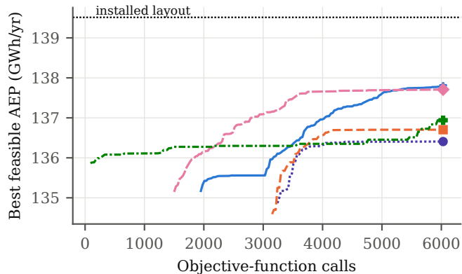
Horns Rev 1, 16 turbines
