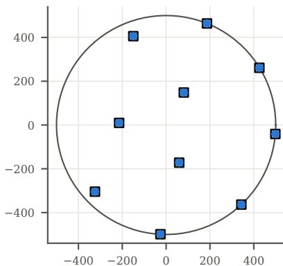
Data Set II, r = 500 m, N = 10 best of all methods: LX-SSA-VNS
