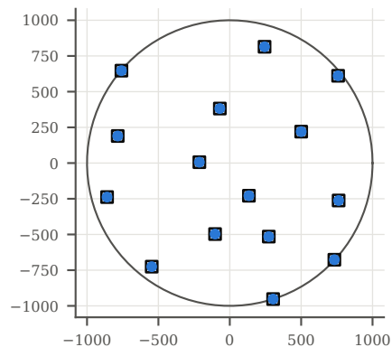
Data Set II, r = 1000 m, N = 15 best of all methods: LX-SSA-VNS
