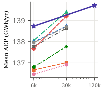
Horns Rev 1, 16 turbines
