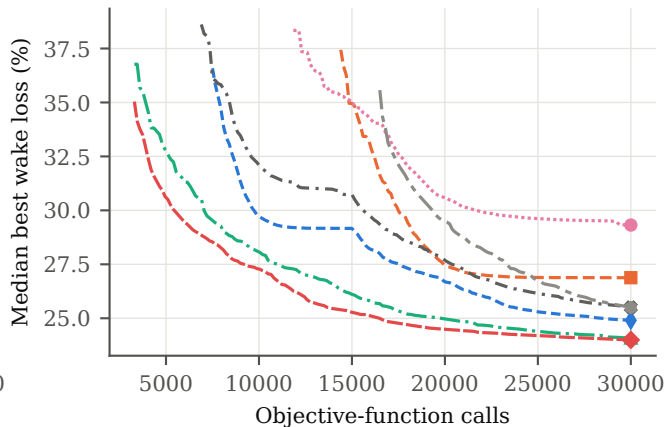
IEA37 CS1, 36 turbines, 30,030 calls
