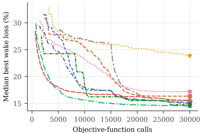
IEA37 CS1, 16 turbines, 30,030 calls
