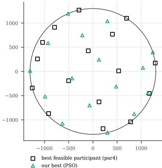
IEA37 CS1, 16 turbines (m)
