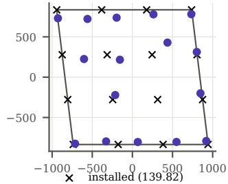
Horns Rev 1, 16 turbines (AEP in GWh/yr)
