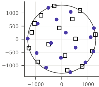
IEA37 CS1, 16 turbines (AEP in MWh)
