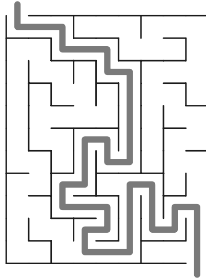
Maze 46
