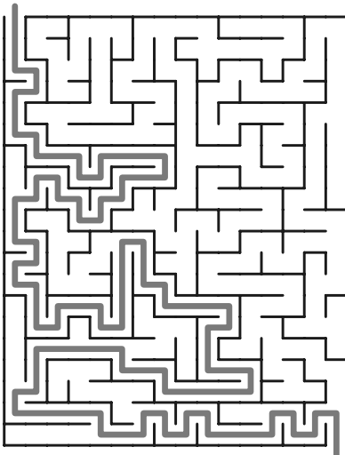
Maze 89
