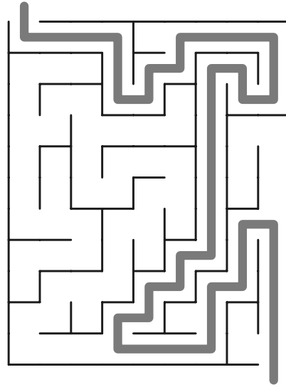
Maze 34
