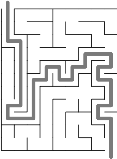
Maze 45
