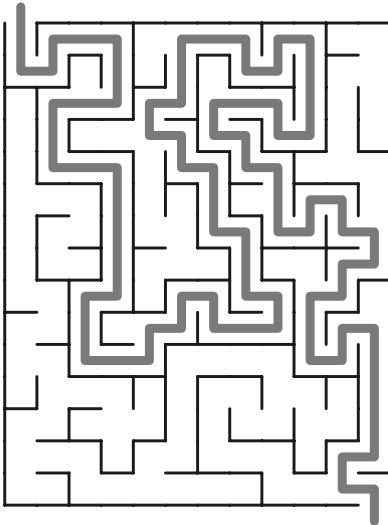
Maze 53
