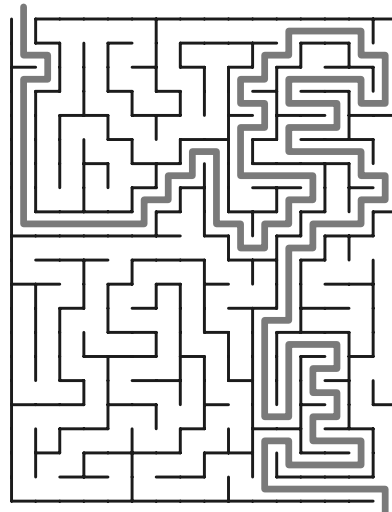
Maze 90
