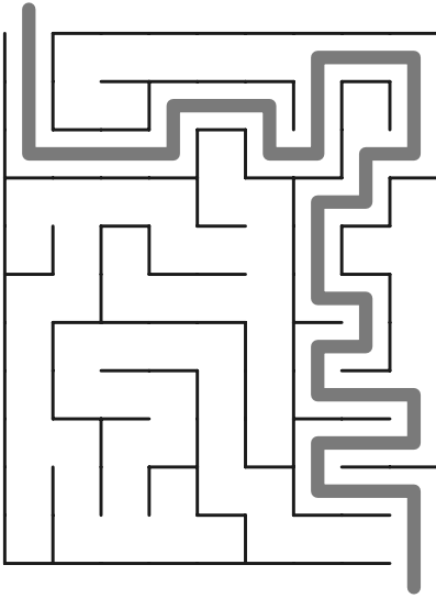
Maze 33
