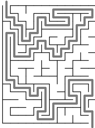
Maze 54
