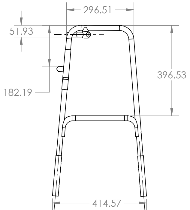
Side View Scale (1:10)
