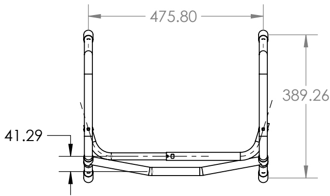
Top View Scale (1:10)
