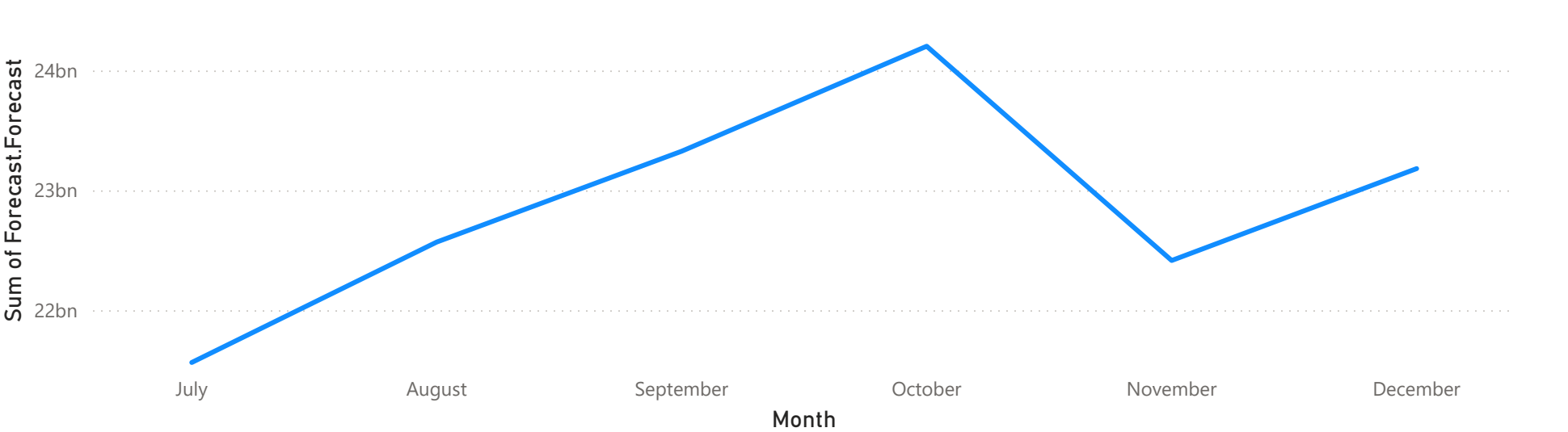
Sum of Forecast.Forecast by Month
