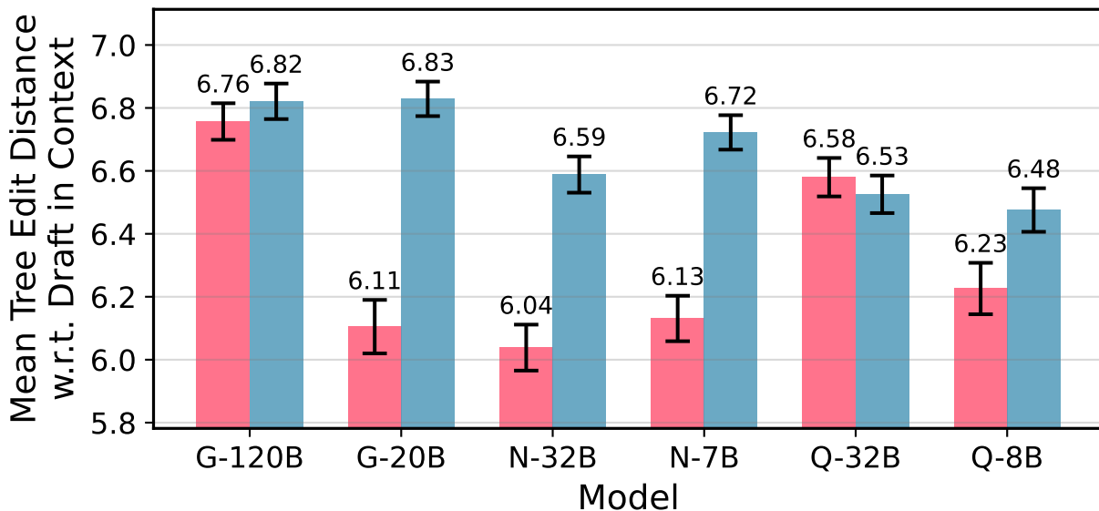
Self-detected Error Awareness
