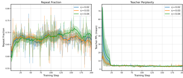
(a) Repetition rate and perplexity curves for \hat{k} = 8 .
