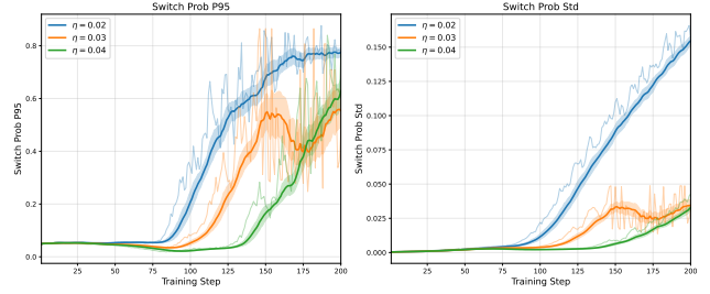
(b) Switch rate curves for \hat{k} = 16 .
