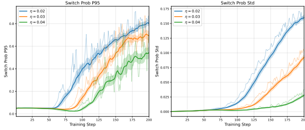
(a) Switch rate curves for \hat{k} = 8 .
