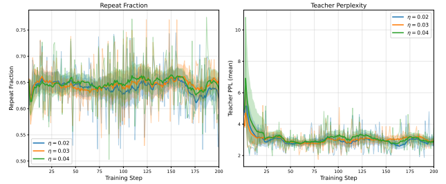
(b) Repetition rate and perplexity curves for \hat{k} = 16 .
