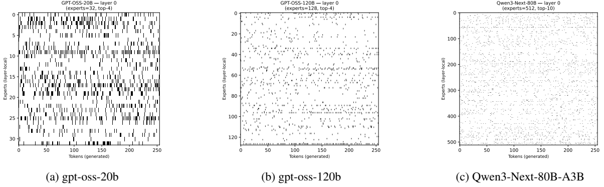
Fig. 2: Set of activated experts in layer 0 throughout the trajectory for each model
