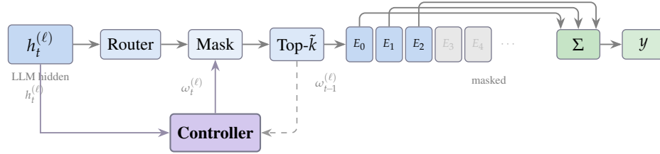
Fig. 3: Controller integration with MoE layer. The controller observes LLM hidden states h_t^{(\ell)} and the current option \omega_{t-1}^{(\ell)} , and outputs a new expert mask \omega_t^{(\ell)} that restricts which experts can be selected by top- \tilde{k} routing. Grayed experts are masked out.
