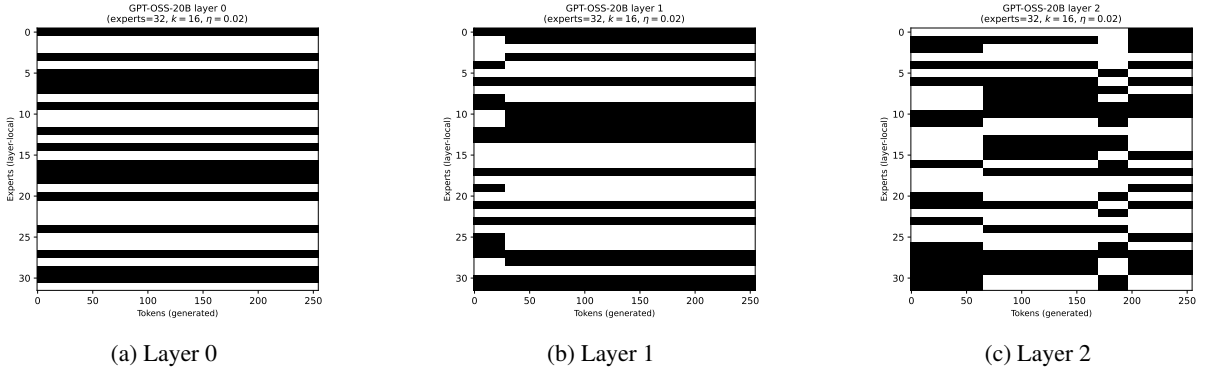
Fig. 7: Options in layer 0, 1, 2 throughout the trajectory with gpt-oss-20b, \hat{k} = 16, \eta = 0.02 .
