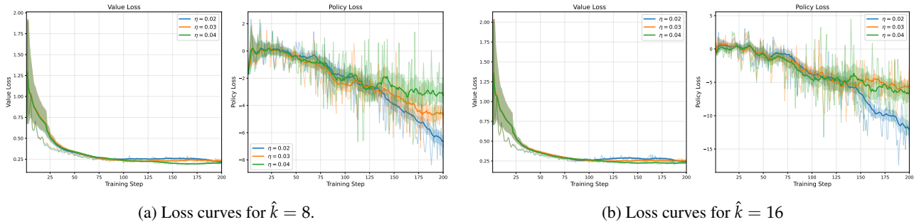
Fig. A1: Loss curves for \hat{k} = 8 and \hat{k} = 16 , respectively. Running averages and confidence bands plotted the same way as in Figure 5.
