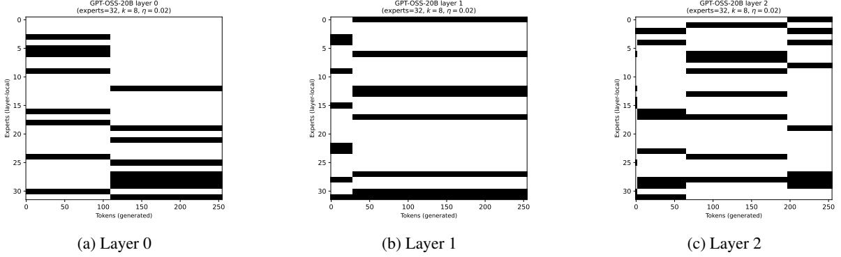
Fig. 6: Options in layer 0, 1, 2 throughout the trajectory with gpt-oss-20b, \hat{k} = 8, \eta = 0.02 .
