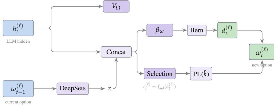
Fig. 4: Controller architecture. The controller takes LLM hidden states h_t^{(\ell)} and the current option \omega_{t-1}^{(\ell)} (a set of \hat{k} expert indices) as inputs. A DeepSets encoder maps \omega_{t-1}^{(\ell)} to a permutation-invariant set embedding z , which is concatenated with h_t^{(\ell)} (after RMSNorm) and fed to the termination head \beta_\omega and the selection head. The state-value head V_\Omega uses h_t^{(\ell)} alone. The selection head is a linear layer initialized from the router weights and produces candidate logits c_t^{(\ell)} = f_{\text{sel}}(h_t^{(\ell)}) , from which \hat{k} experts are sampled via the Plackett–Luce distribution. If the Bernoulli sample d_t^{(\ell)} = 1 , the newly sampled option replaces the current one; otherwise the current option persists.
