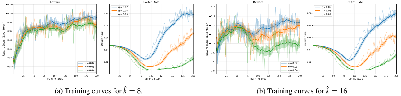
Fig. 5: Reward curves and switch rate curves for one training run. We present the running averages over sliding windows of size 20. The shaded bands show bootstrap 95% confidence intervals for the running mean, computed by resampling (with replacement, 1000 times) within a sliding window of 20 steps and taking the 2.5th and 97.5th percentiles of the resampled means.
