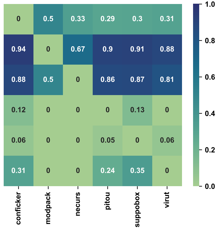
False Positive Ratio
