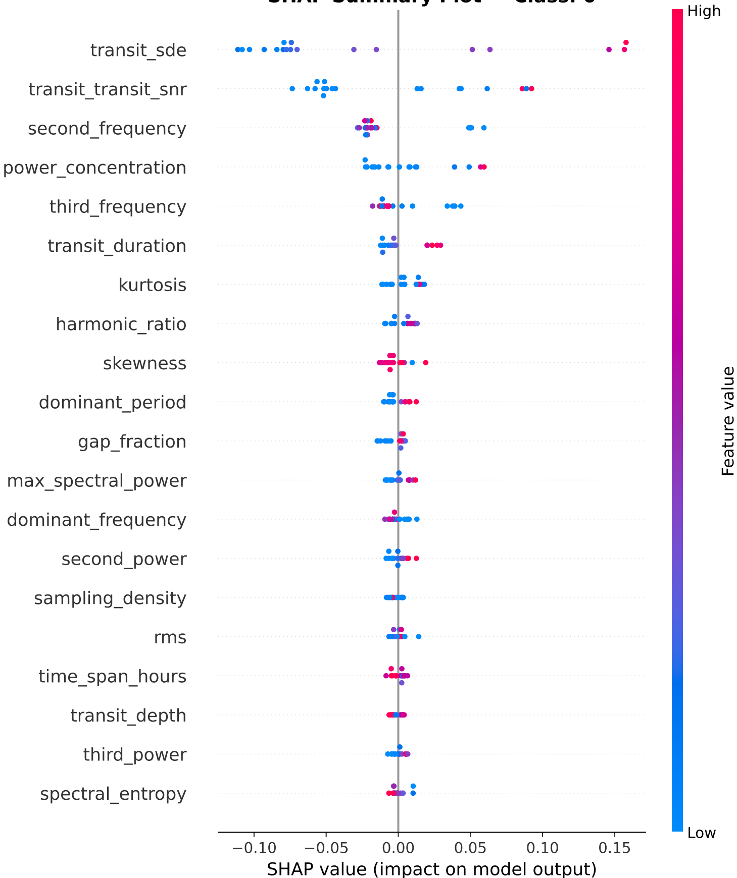
SHAP Summary Plot — Class: 0
