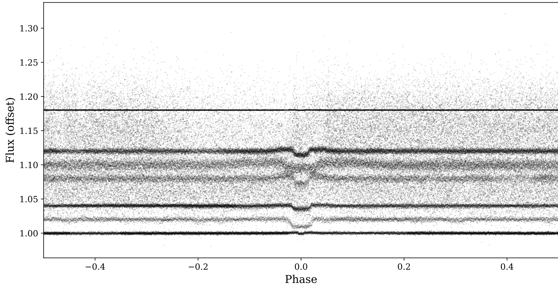
All Candidate Phase-folded Transits
