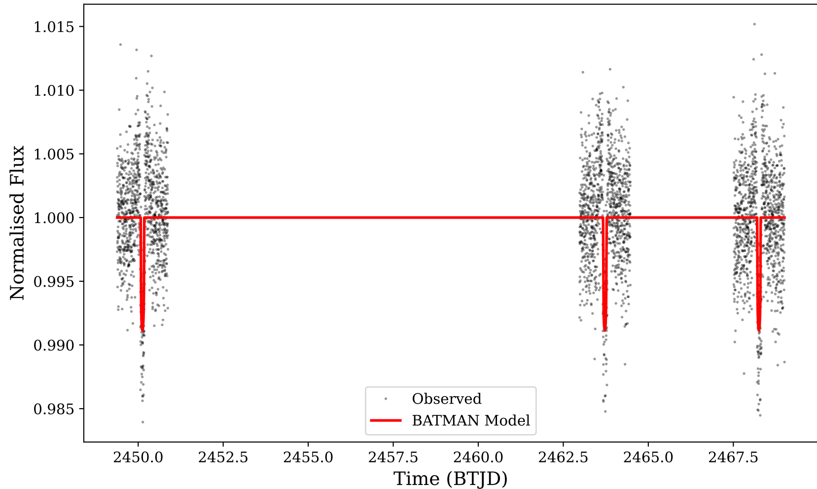
TIC 262662119 — Observed vs BATMAN Model
