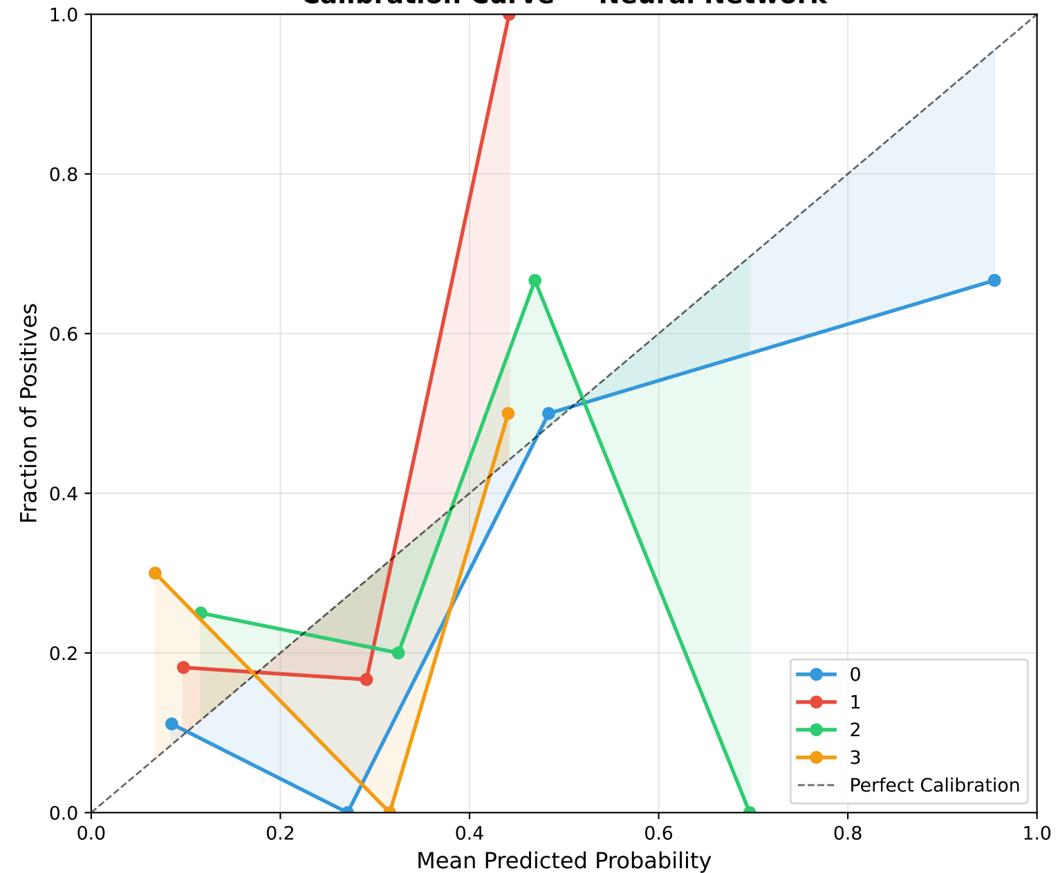
Calibration Curve — Neural Network
