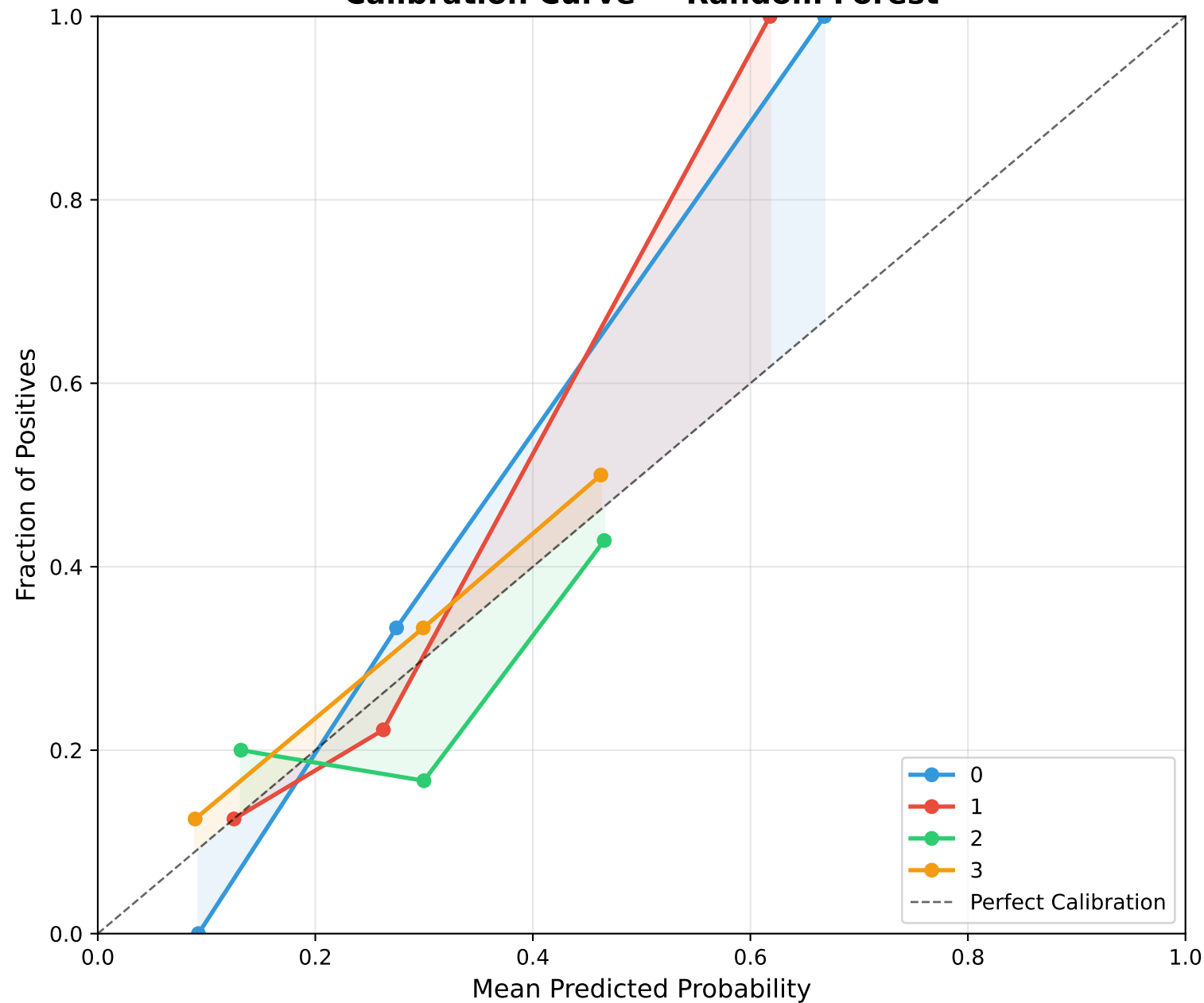
Calibration Curve — Random Forest
