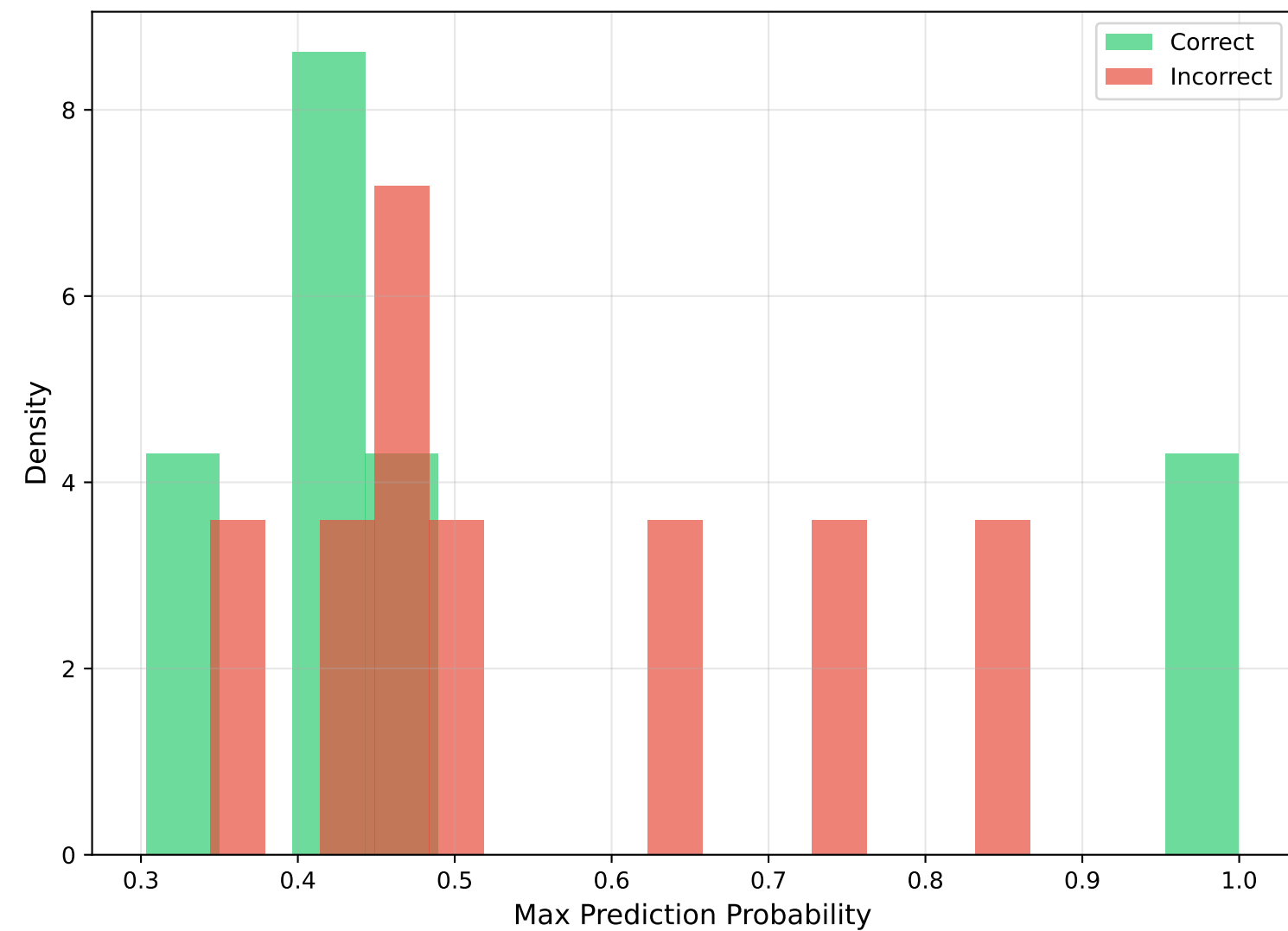
NN Confidence: Correct vs Incorrect
