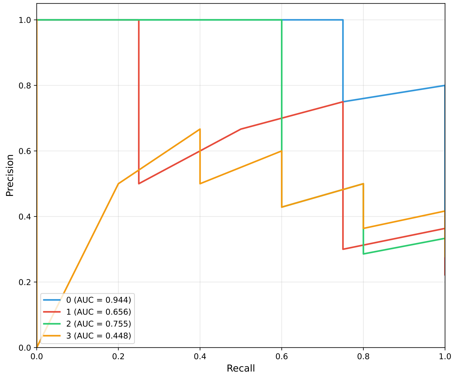
Precision-Recall Curves — Random Forest
