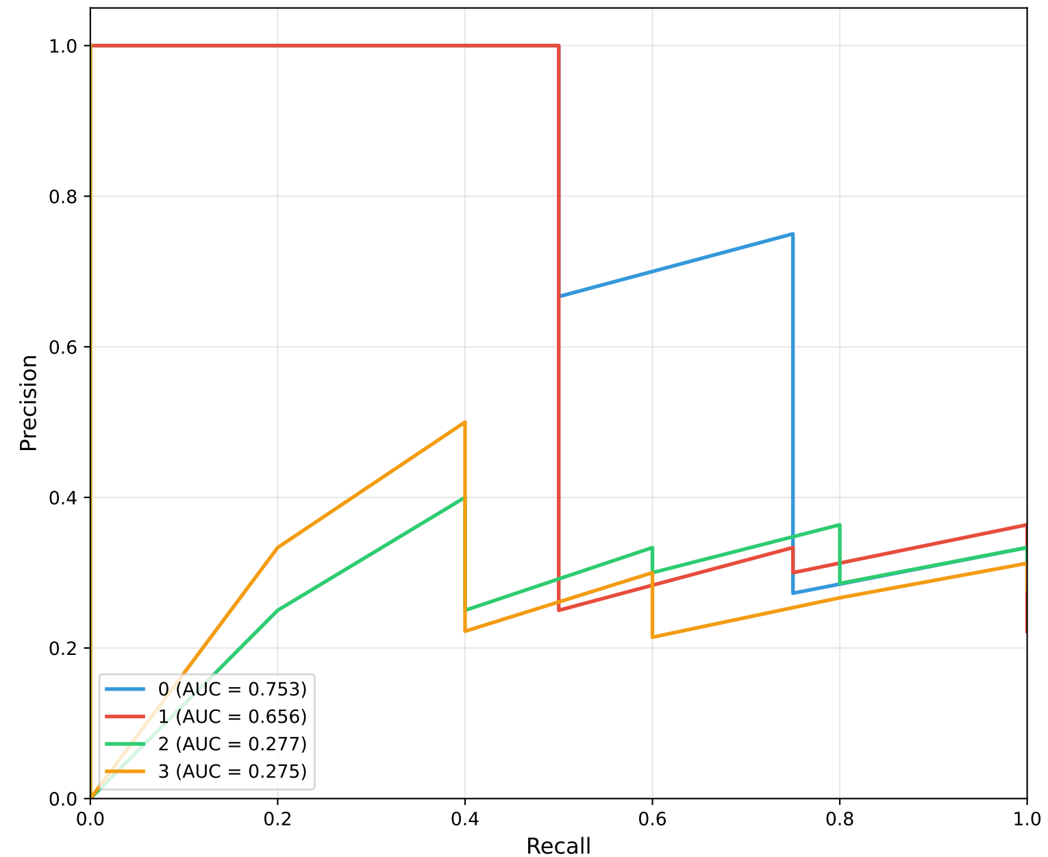
Precision-Recall Curves — Neural Network
