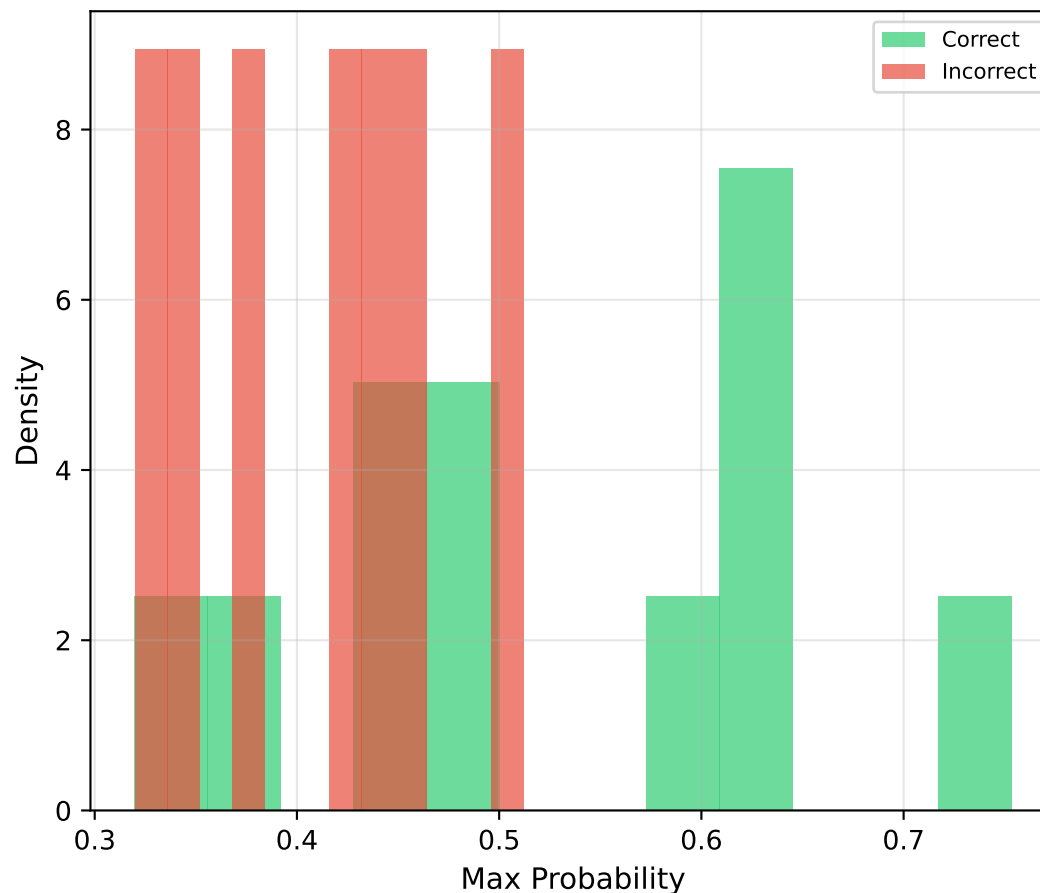
Confidence Distribution (RF)
