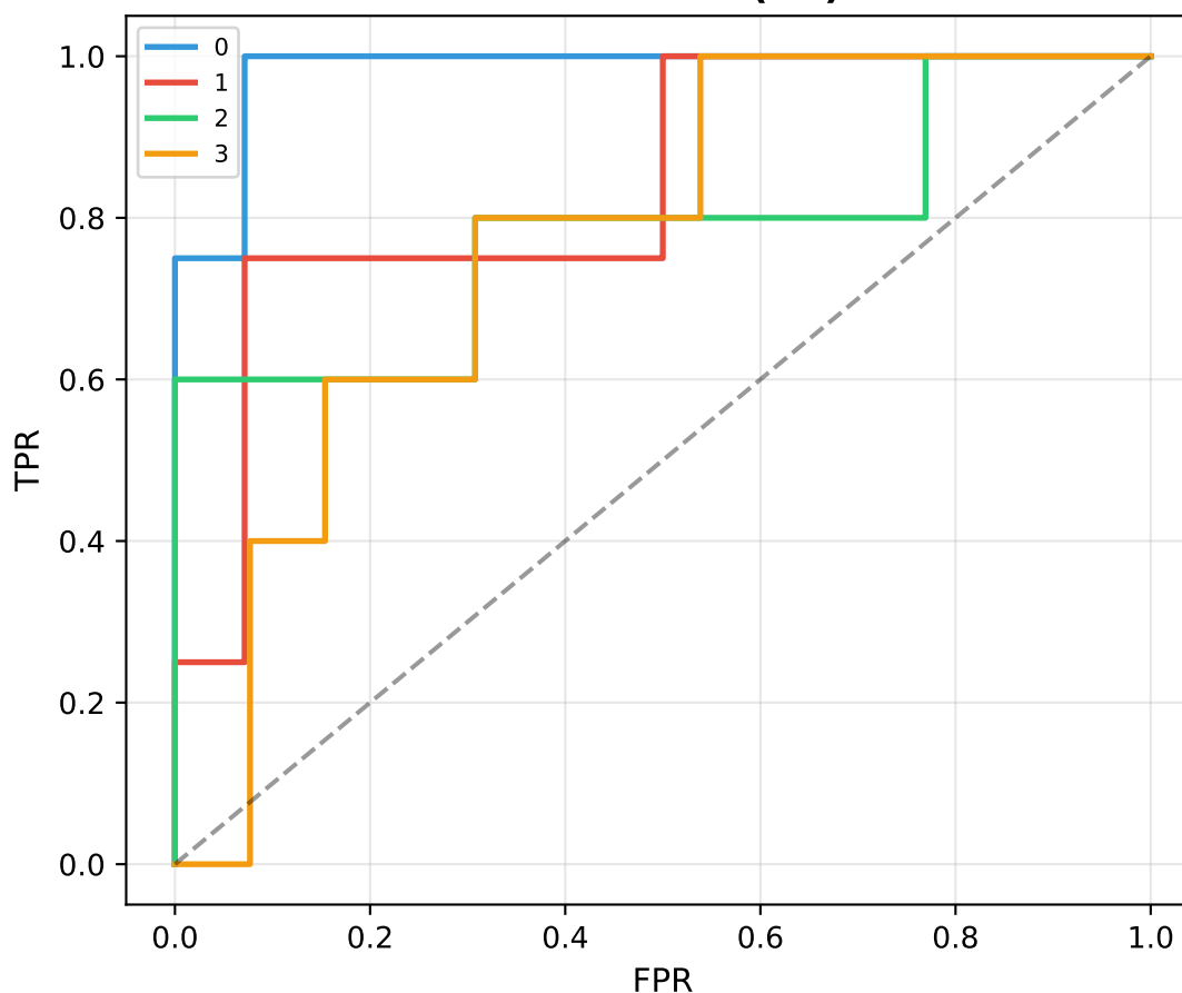
ROC Curves (RF)
