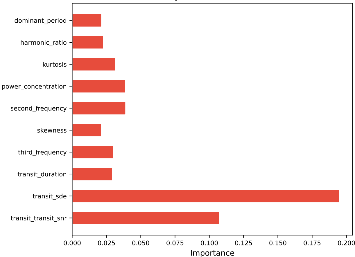
Top Features — NN
