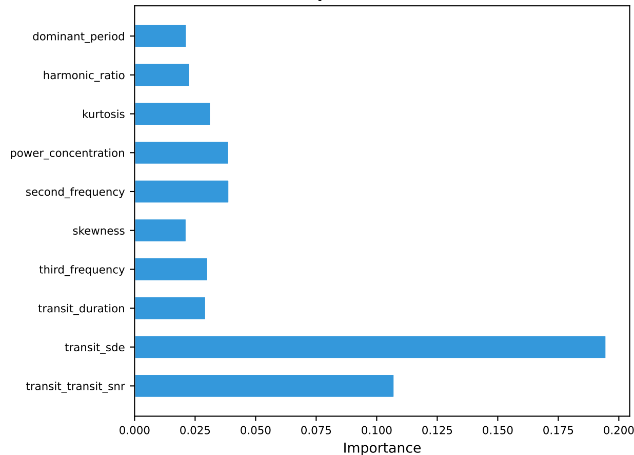
Top Features — RF
