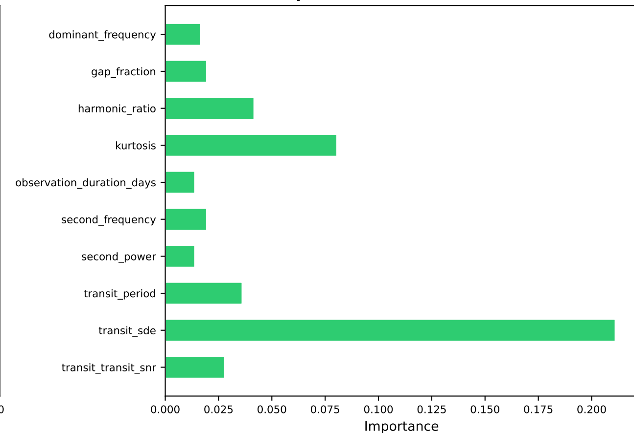
Top Features — Permutation
