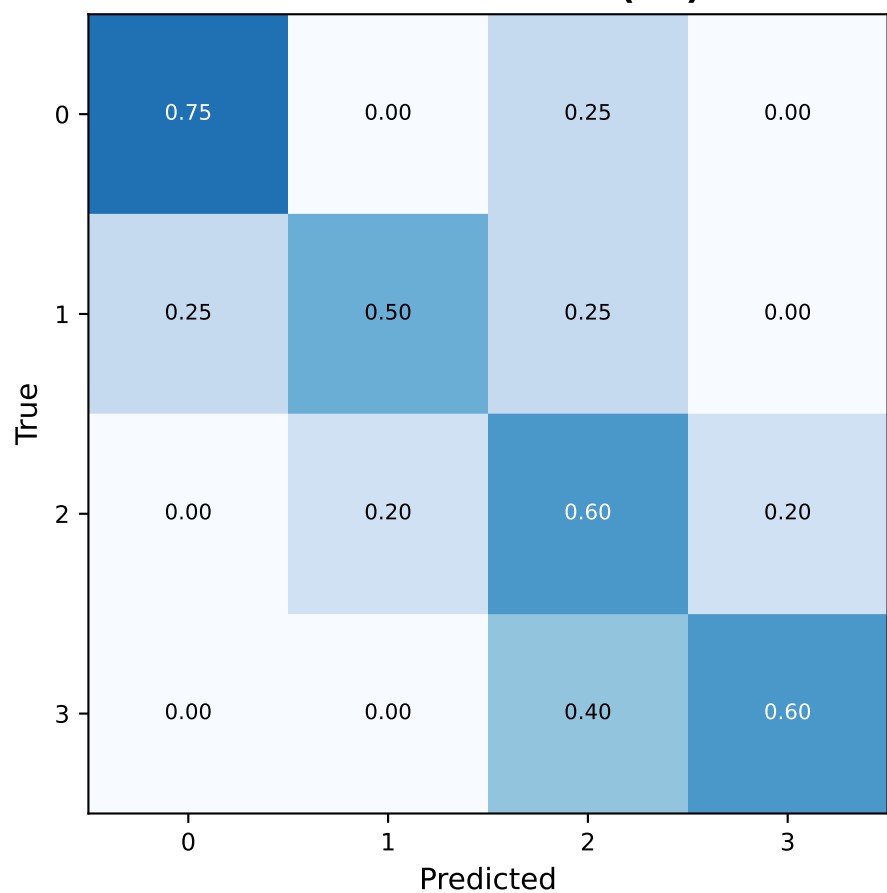
Confusion Matrix (RF)
