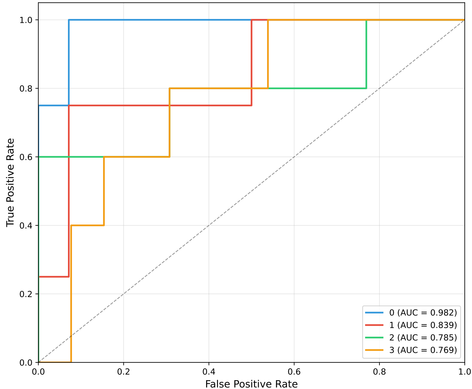
ROC Curves — Random Forest
