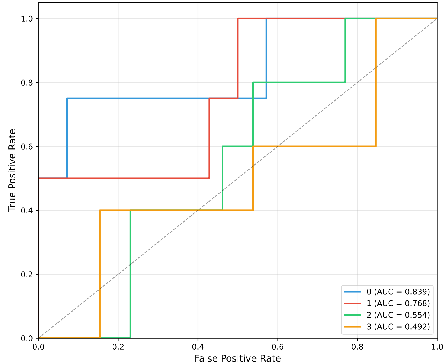
ROC Curves — Neural Network
