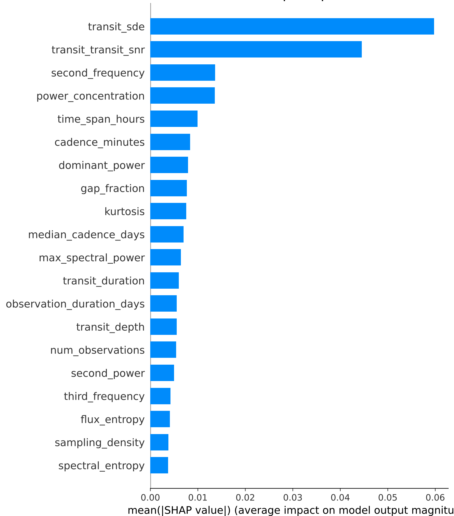
SHAP Mean |SHAP| — Class: 1
