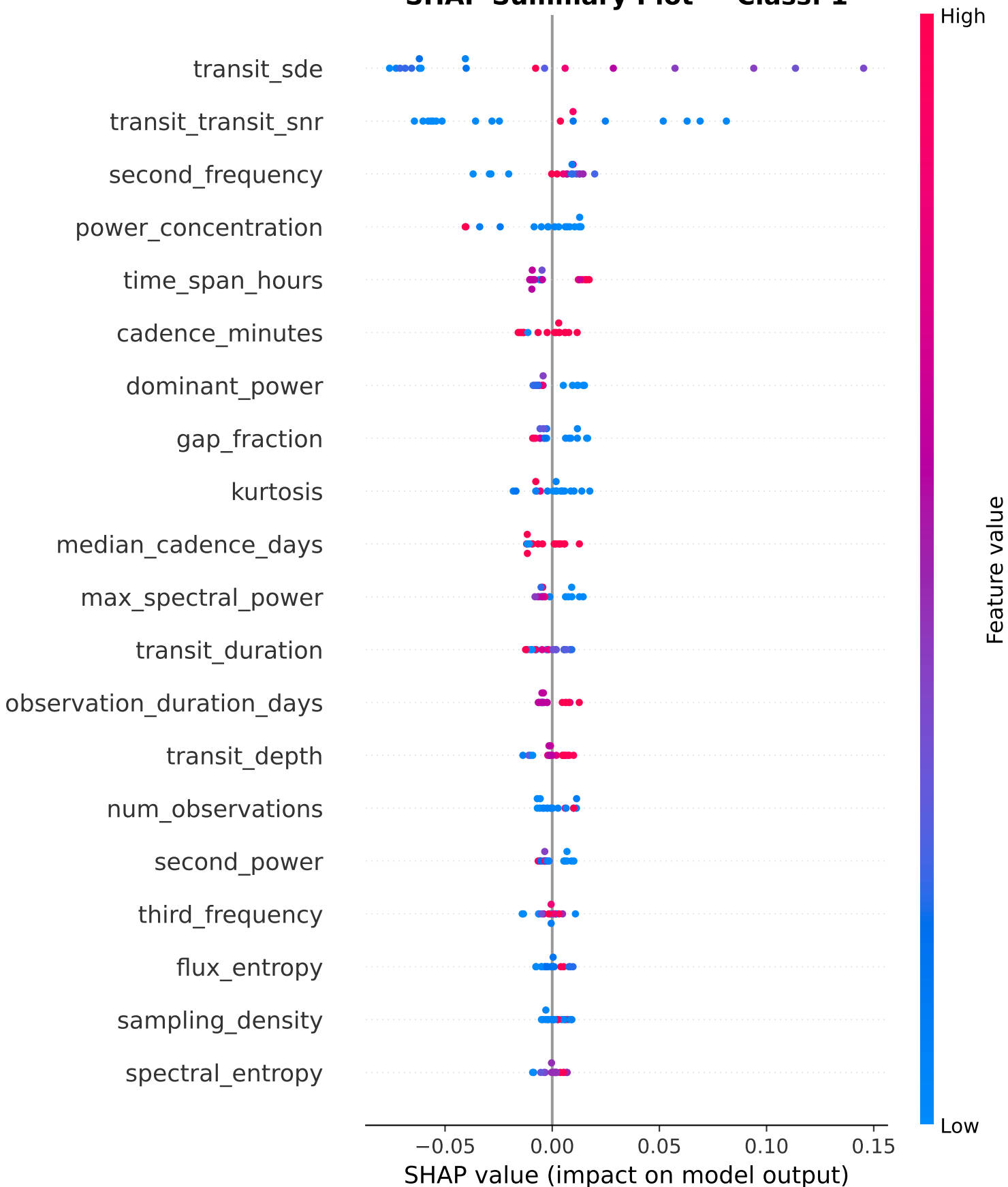
SHAP Summary Plot — Class: 1
