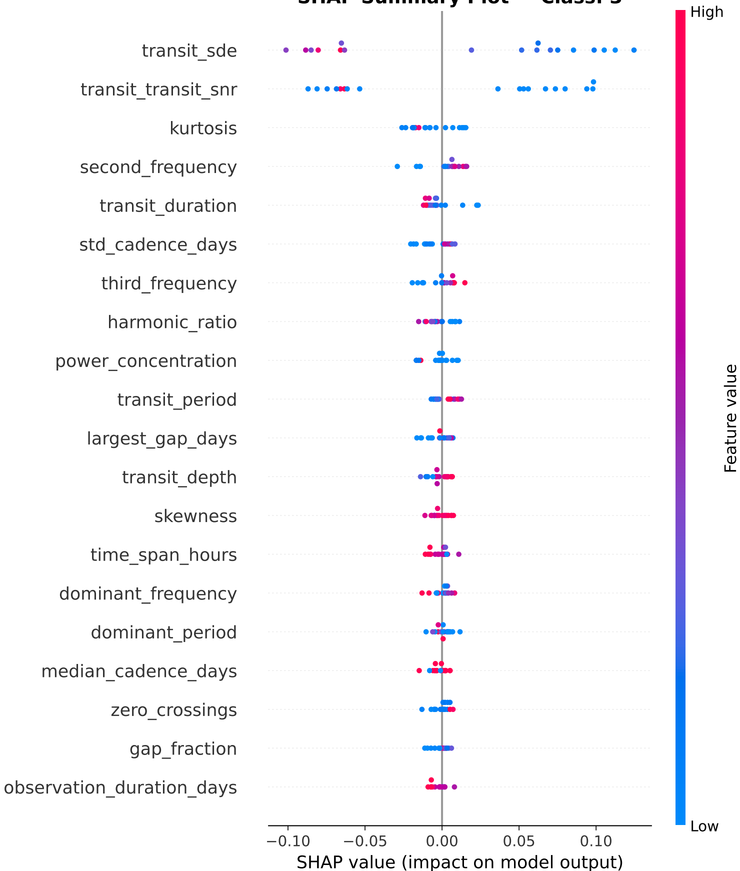
SHAP Summary Plot — Class: 3
