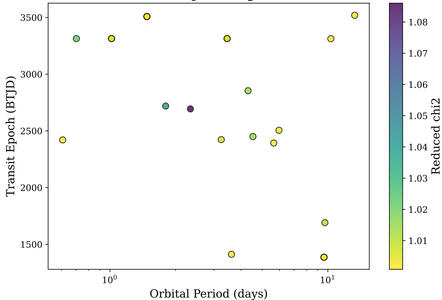
Period-Epoch Diagram
