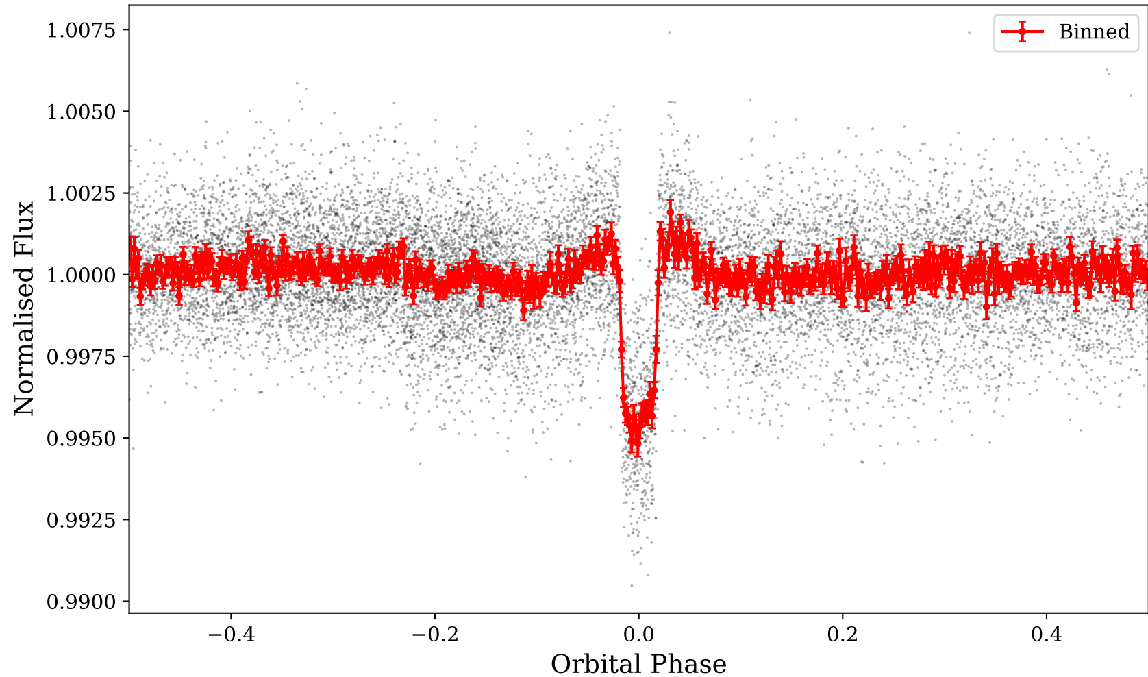
TIC 152476657 — Phase-folded Light Curve (P=3.6106 d)
