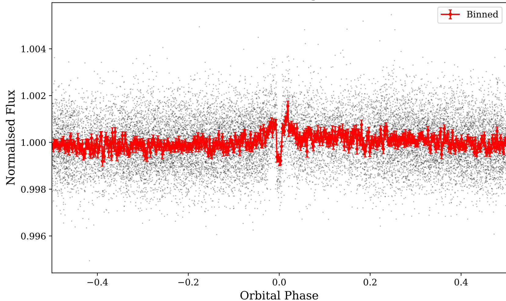
TIC 158002130 — Phase-folded Light Curve (P=9.6968 d)
