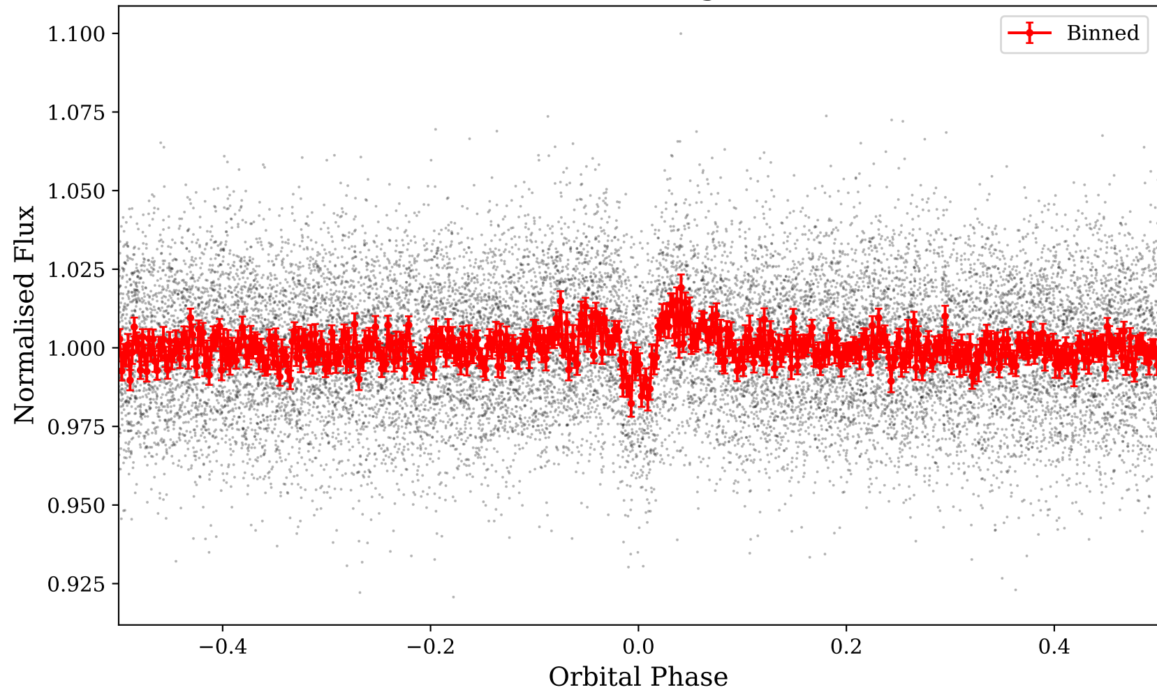
TIC 27318774 — Phase-folded Light Curve (P=3.2424 d)
