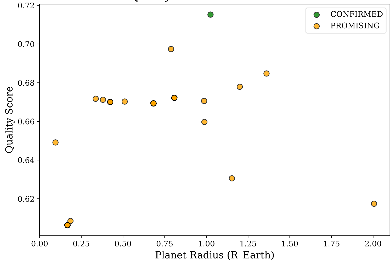
Quality Score vs Planet Radius
