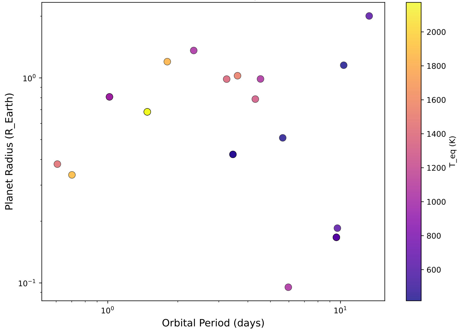
Radius-Period Diagram
