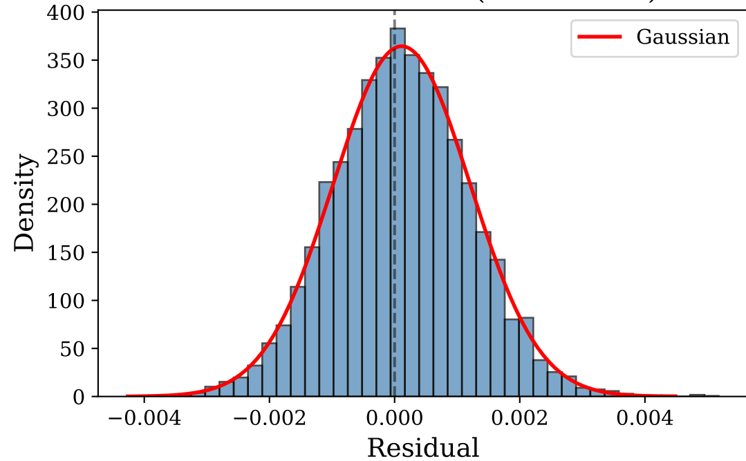
Residual Distribution ( \sigma=0.001094 )
