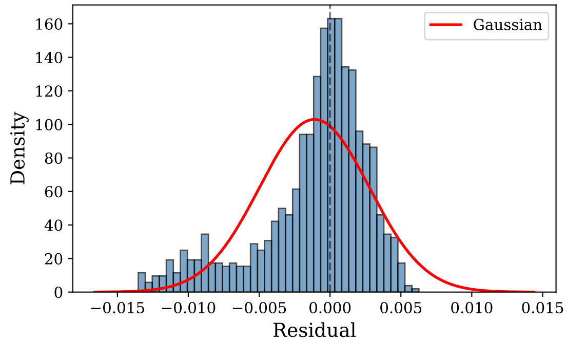
Residual Distribution ( \sigma=0.003874 )
