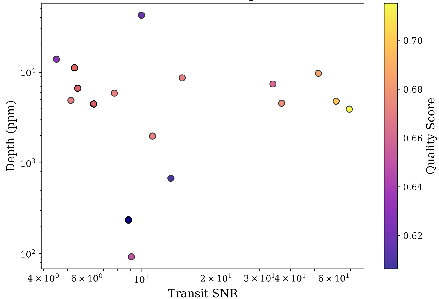
SNR vs Transit Depth
