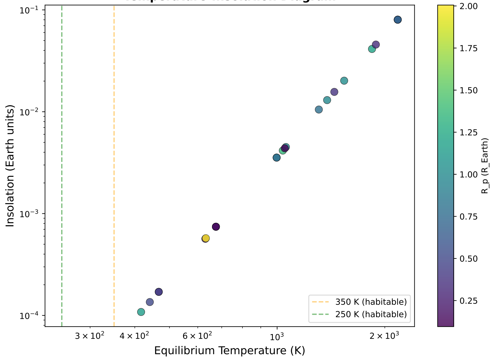
Temperature-Insolation Diagram
