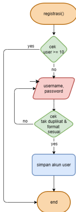
gambar 2.13 Flowchart registrasi user
