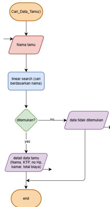
gambar 2.8 Flowchart Cek Data Tamu
