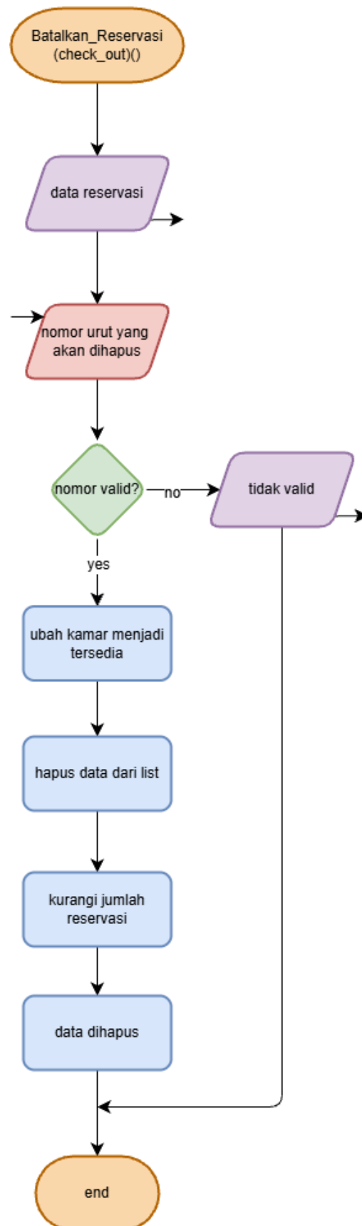
gambar 2.6 Flowchart Batalkan Reservasi (Delete)
