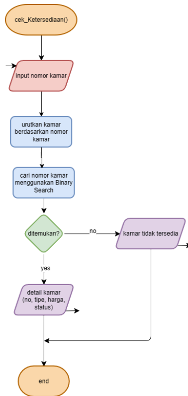
gambar 2.9 Flowchart Cek Ketersediaan
