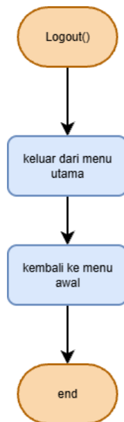
gambar 2.11 Flowchart Logout
