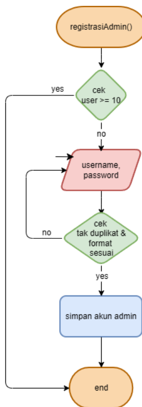
gambar 2.14 Flowchart registrasi admin
