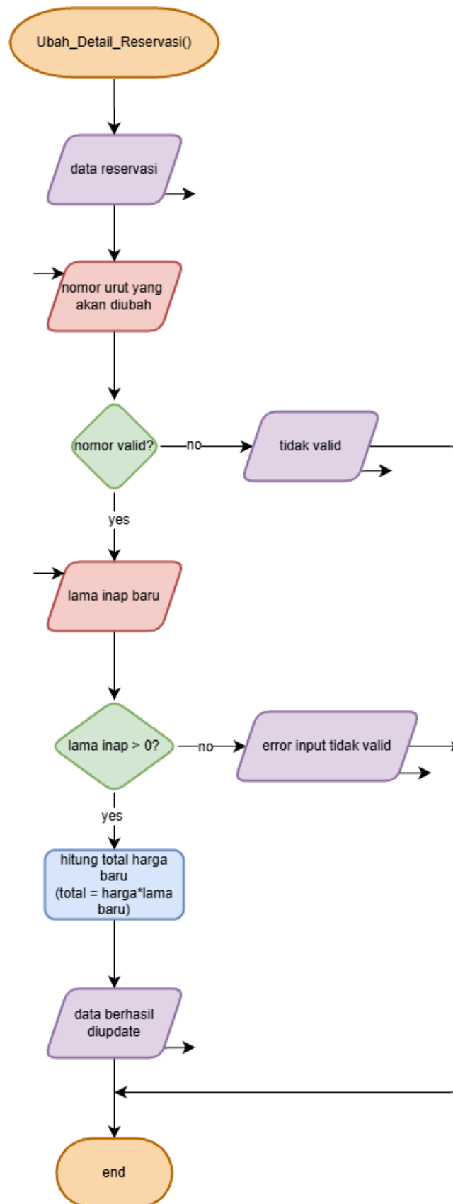
gambar 2.5 Flowchart Ubah Detail Reservasi (Update)
