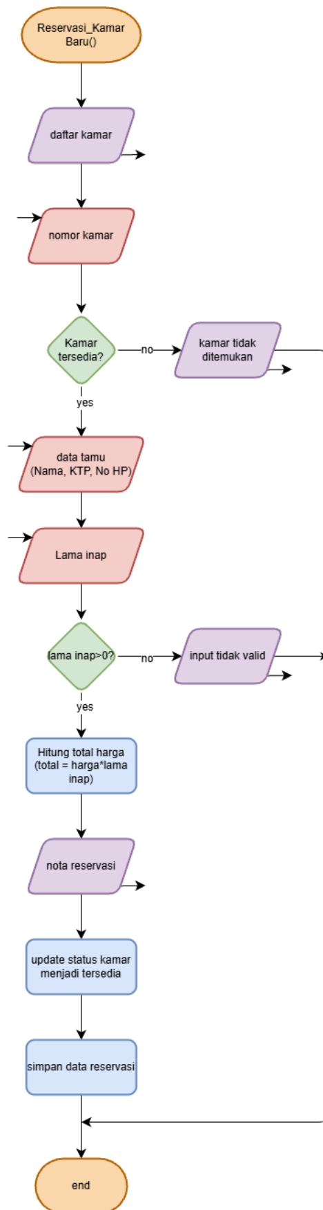
gambar 2.3 Flowchart Reservasi Kamar Baru
