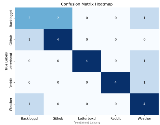
Figure 6: The confusion matrix for the Random Forest model with the given dataset
